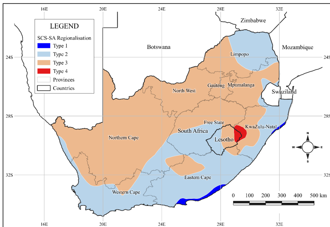
Figure 2.9: Regionalisation of synthetic rainfall distributions in southern Africa (Weddepohl, 1988)
