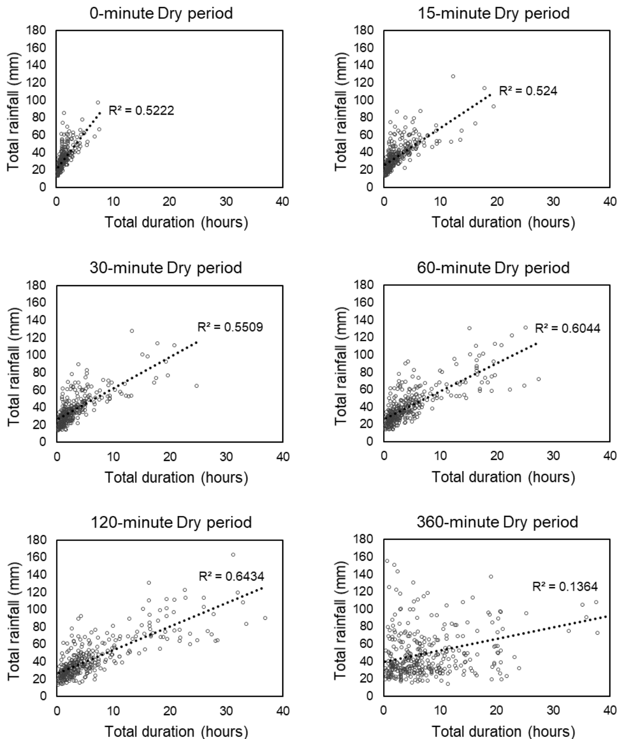
Figure 4.1 Correlation between total rainfall and duration for different MDP criterion
