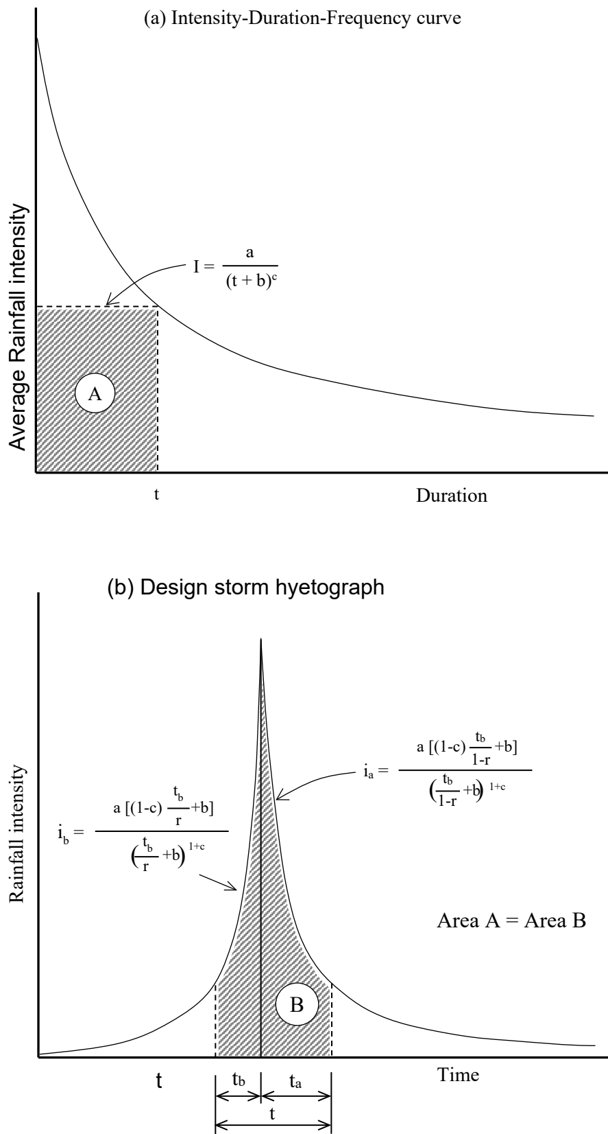
Figure 2.3: Chicago Design Storm (Watson, 1981)
